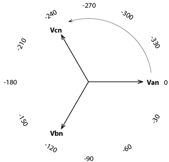
NEGATIVE PHASE ANGLES (LAGGING) GE-UR Relays Manta (Optional) Test-Sets
